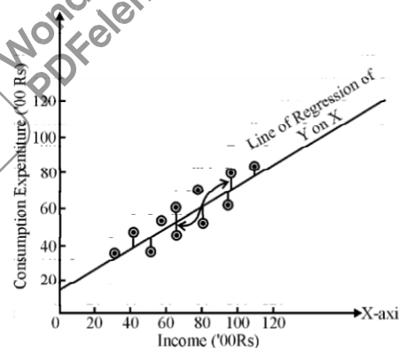
Fig. 3.3 Scatter Regression Line and Representing 'e'
