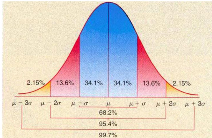
Fig. 4.4 Normal Curve Showing Areas at Different Distances from the Mean
