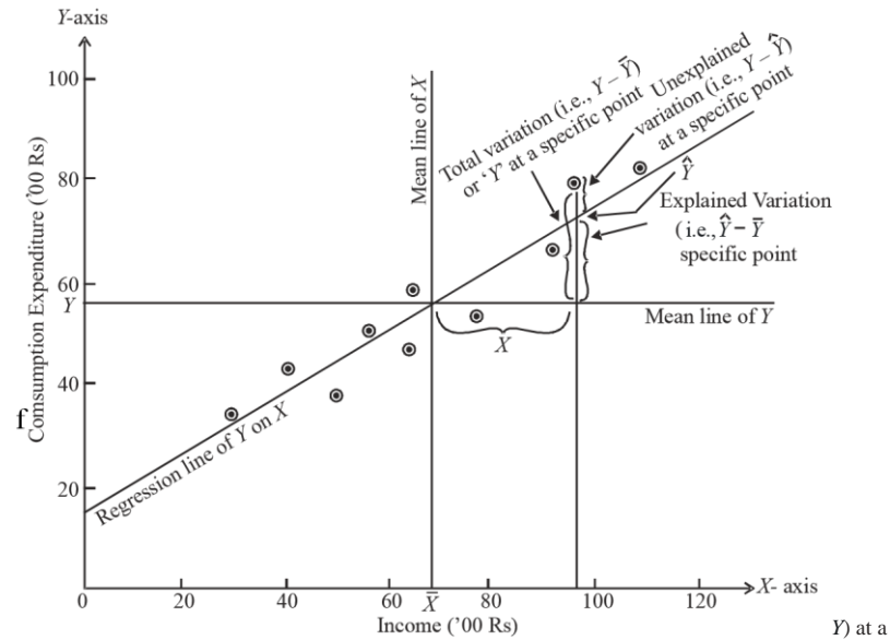
Fig. 3.1 Diagram Showing Total, Explained and Unexplained Variations
