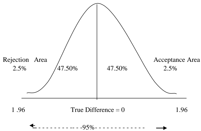
Fig. 4.6 A Two-Tailed Test at 0.05 Levels (2.5 Per Cent at Each Level)
