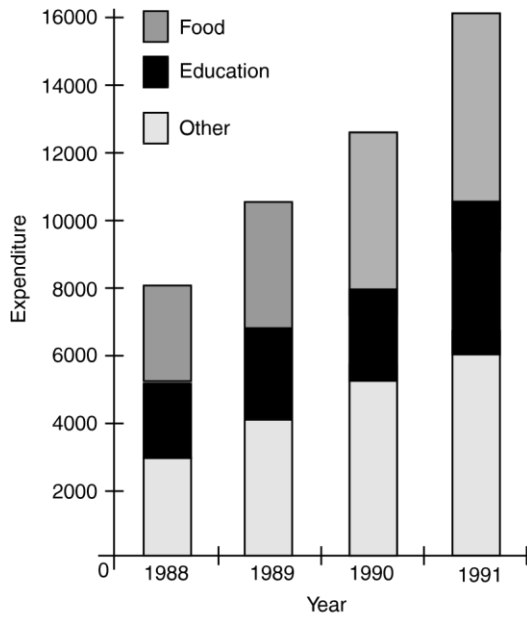
Fig. 1.2 Sub-Divided Bar Diagram
